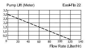
Pump Lift & Flow Rate Chart
